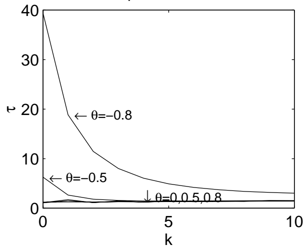
Figure 1: \tau_T(k)
